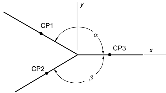
Figure 12.3.4 Kutta condition—second method
