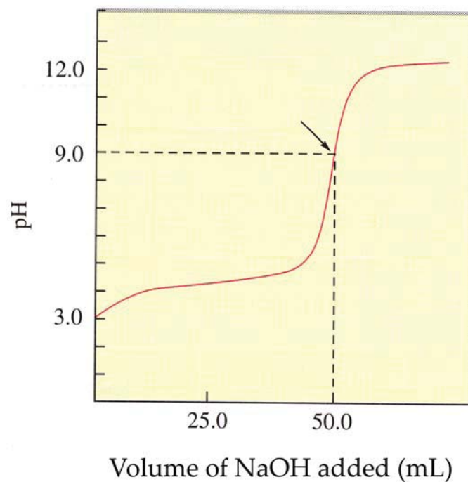
Figure 5- 2: Titration curve
