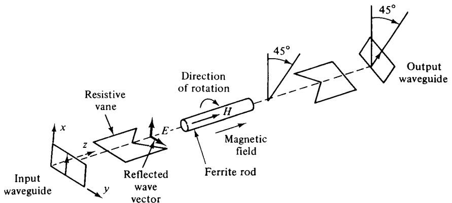
Figure 4-6-5 Faraday-rotation isolator.
