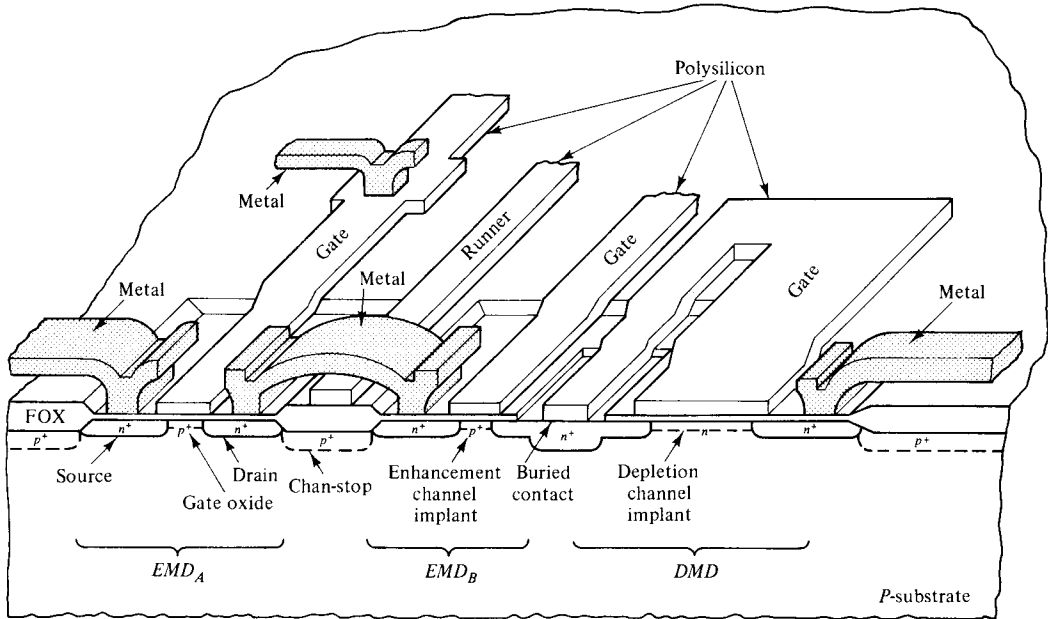
Figure 6-5-1 Three-dimensional view of an NMOS logic circuit. (After Parrillo [13]; reprinted by permission of the Bell Laboratory.)
