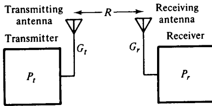
Figure 2-4-2 Electromagnetic energy transmission between two antennas.
