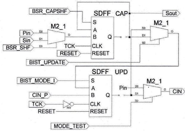
Fig.7 BIST-BSR Input cell
