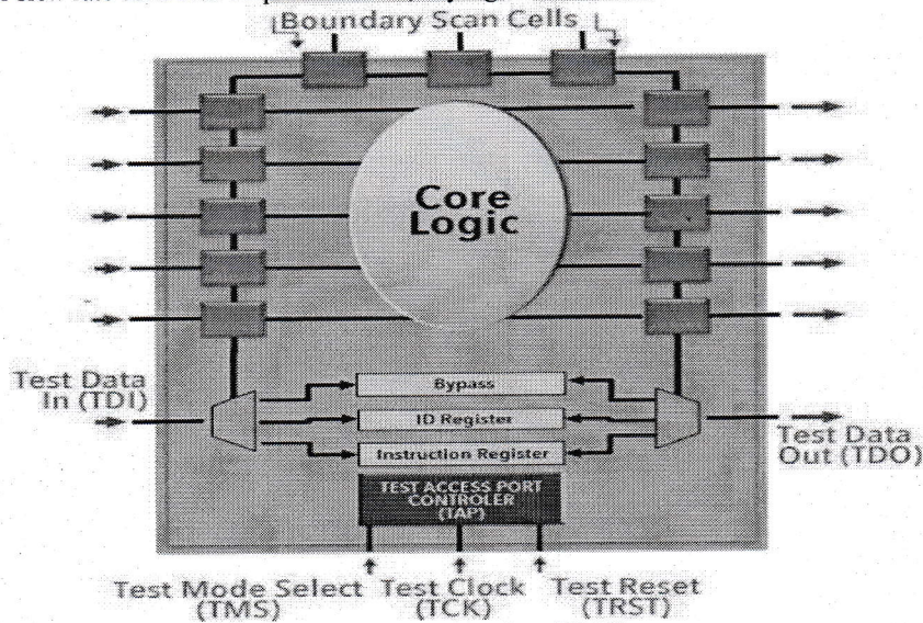
Fig.13 Boundary Scan I/O[6]
