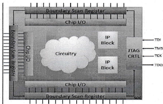
Fig.14 Boundary Scan I/O[6]
