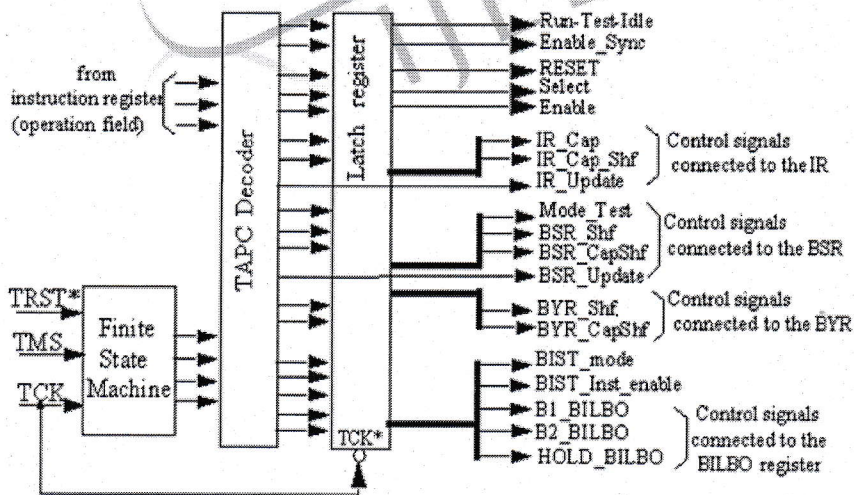
Fig.9 Block diagram of TAP Controller
