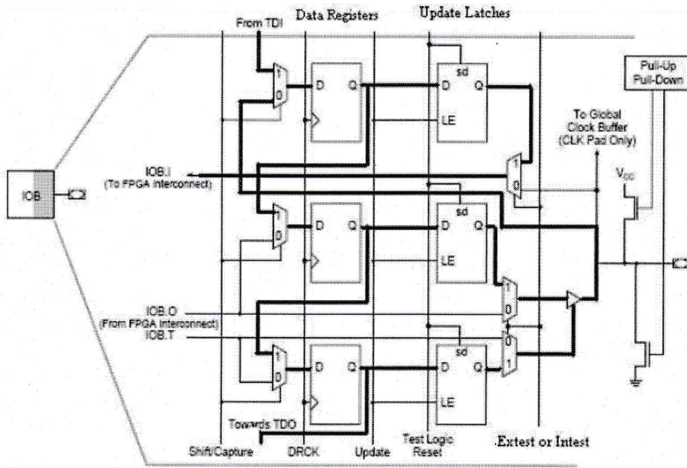
Fig.2 Tested Data lines in an input cell
