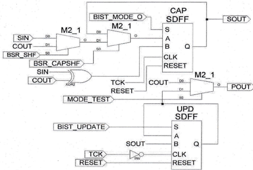
Fig.8 BIST-BSR Output cell
