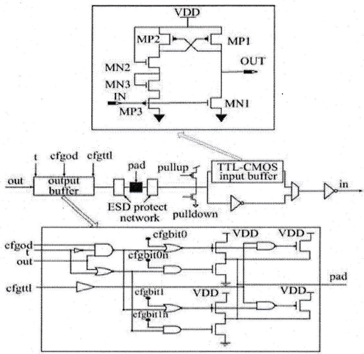
Fig.6 Programmable IO buffers
