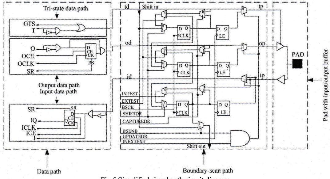
Fig.5 Simplified signal path circuit diagram
