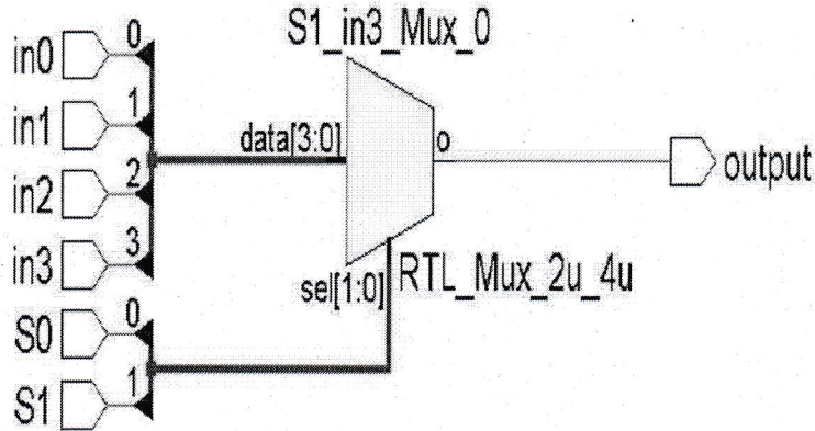
Fig.10 Design of Low power 4x1 Mux
