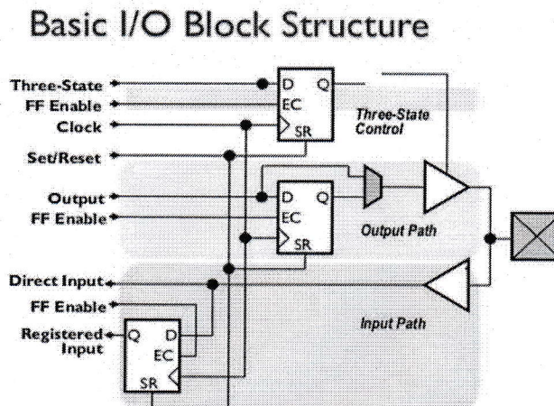
Fig.11 Basic I/O structure[6]
