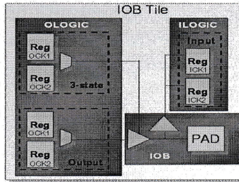
Fig.15 Spartan 6 IOB structure[6]
